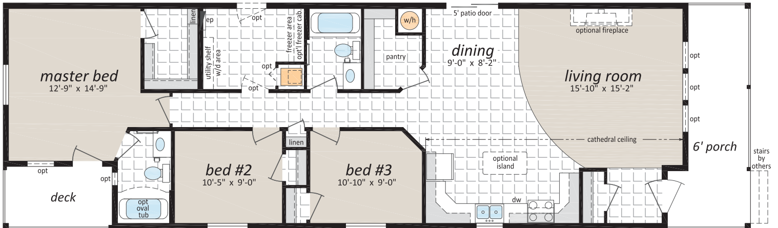
CC - 226601 22' x 72' • 1,584 sq. ft.
