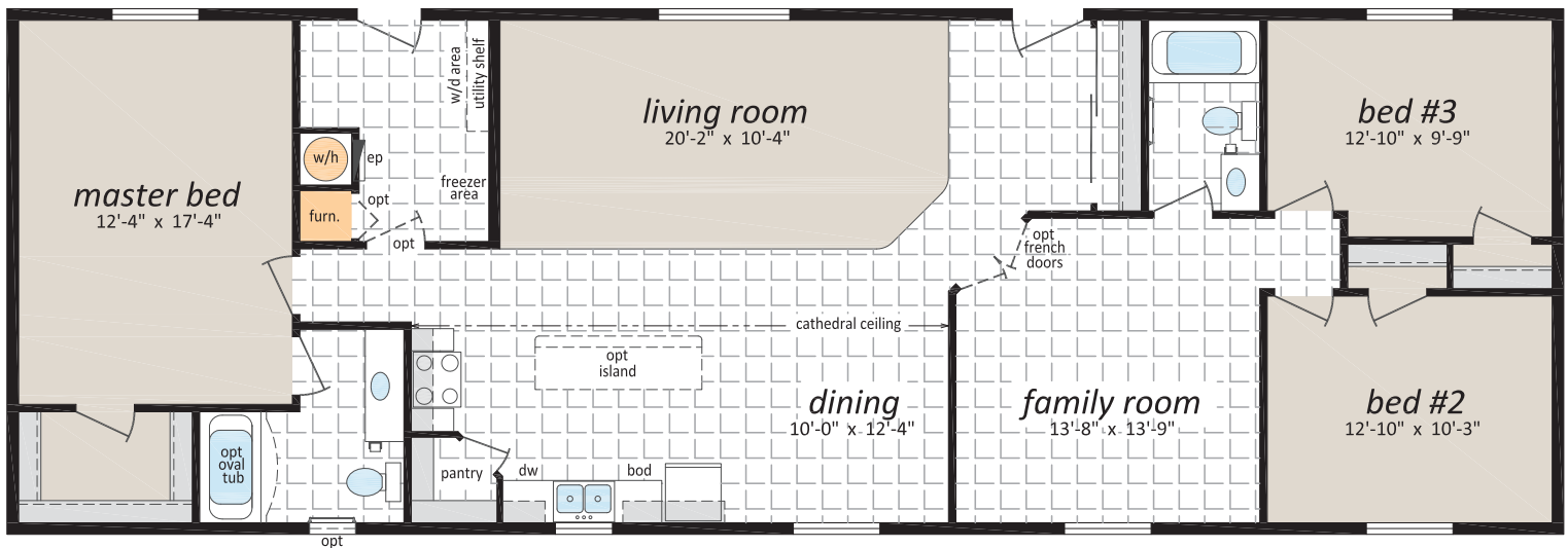
ML-247 24' x 70' - 1,680 sq. ft. 3 Beds, 2 Baths
