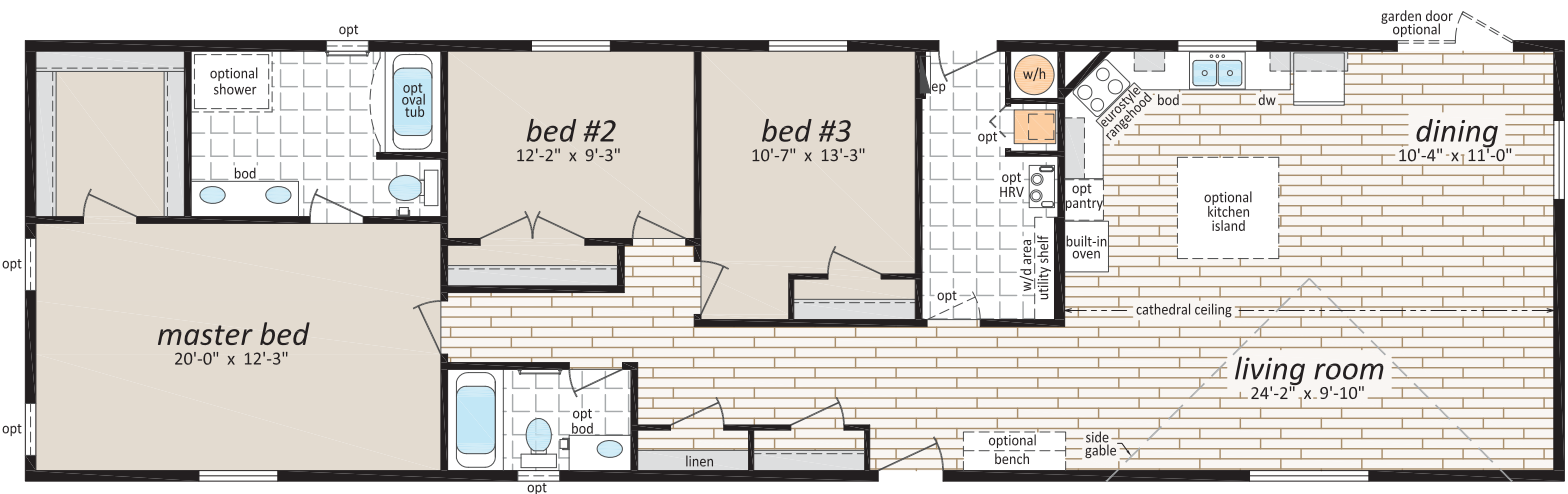
MT-227604 22' x 76' - 1,672 SQ.FT. 3 BEDS, 2 BATHS
