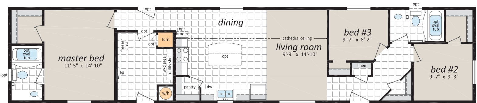
ML-1610 16' x 76' - 1,216 sq. ft. 3 Beds, 2 Bath
